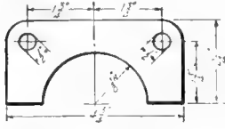
Fig. 15. Detail of the rear support
